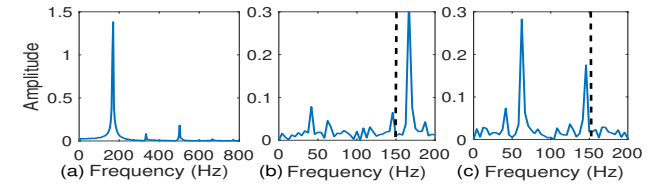
Figure 16: We restore the vibration signal with Supersampling Rate Reconstruction .
